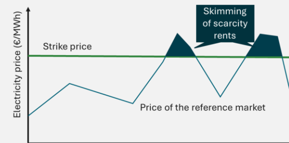
Figure: Working of reliability options
